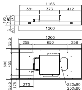
SALIERI 120 (25Kg) HERA 120 (25Kg)
