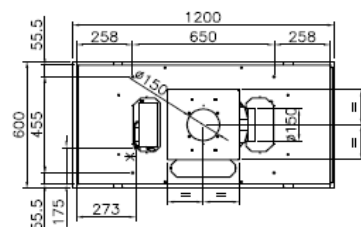
SALIERI 120 (25Kg) HERA 120 (25Kg)
