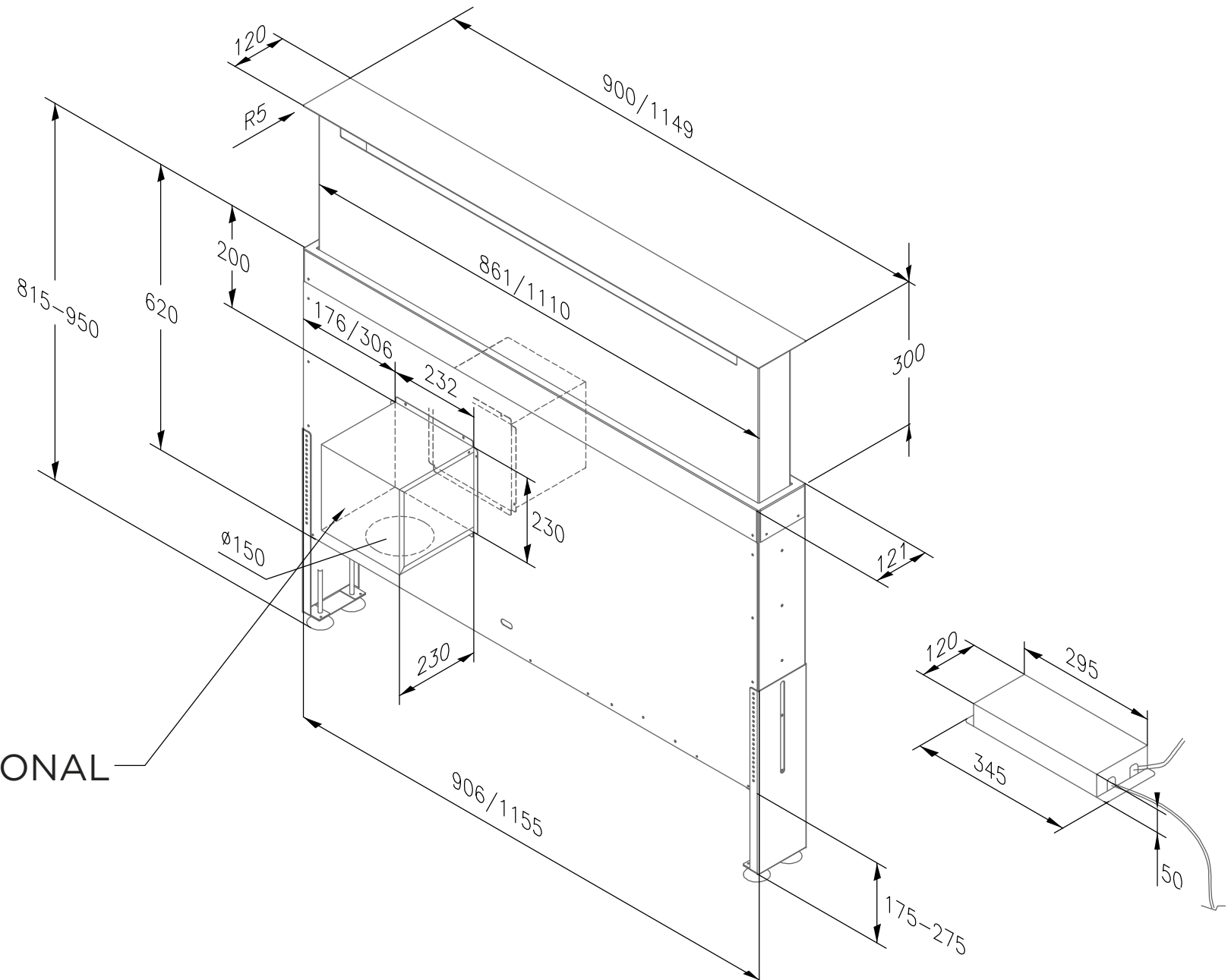
FORATURA PIANO CON KPL CUTOUT COUNTERTOP WITH KPL
