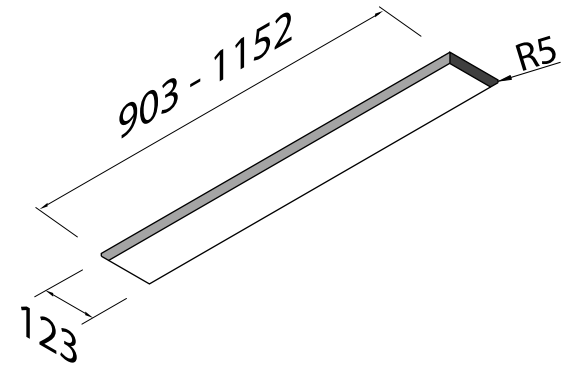
FORATURA PIANO CON KPL CUTOUT COUNTERTOP WITH KPL
